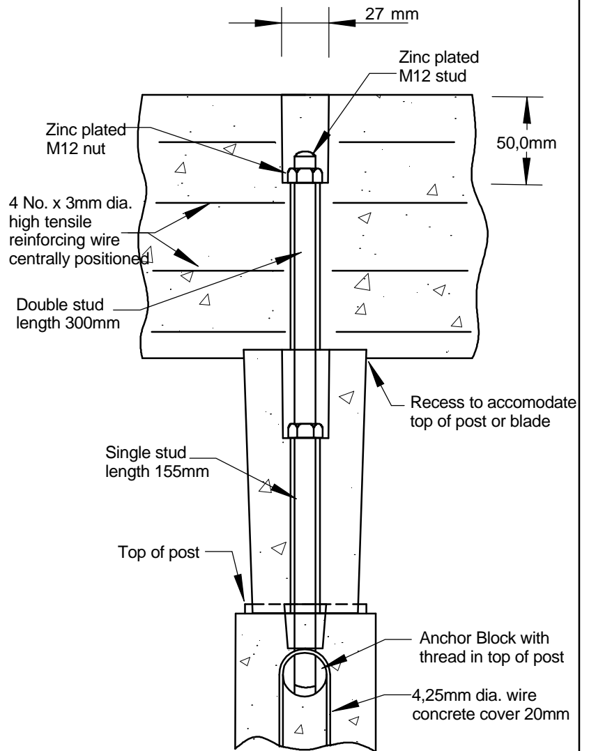
SIDE ELEVATION
